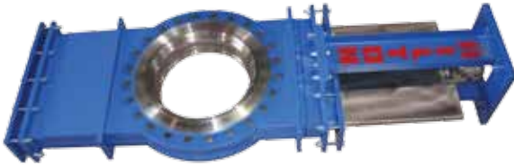
24" Thru-Port Knife Gate, 150 psi, Replaceable Bi-directional Metal Seats, Teflon Internal Cavity Filler, Tianjin Chemical China & GE Plastics Mississippi
